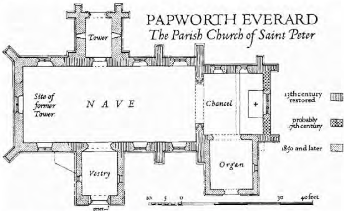
Figure 9 - Plan of the Parish Church of St Peter (An Inventory of the Historical Monuments in the County of Cambridgeshire, Volume 1, West Cambridgeshire).
